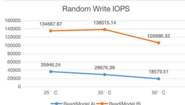
Fig. 3. IOPS for Flash Read/Write Operations.
